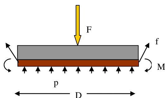
Fig 4: Free body diagram of plastic diaphragm
