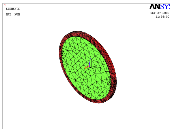
Fig 5: ANSYS model of piezoelectric
