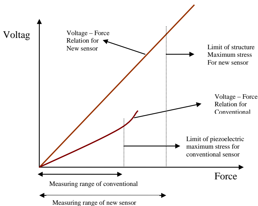
Fig 10: Voltage-Force diagram
