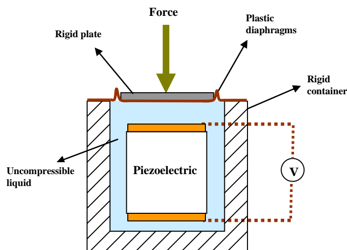
Fig 2: New proposed sensor structure
