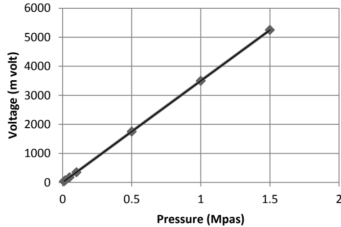
Fig 6: Voltage-pressure diagram
