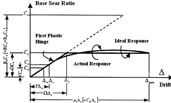
Fig 1: General behavior of a conventional structure (Tasnimi et al. (2007)).
