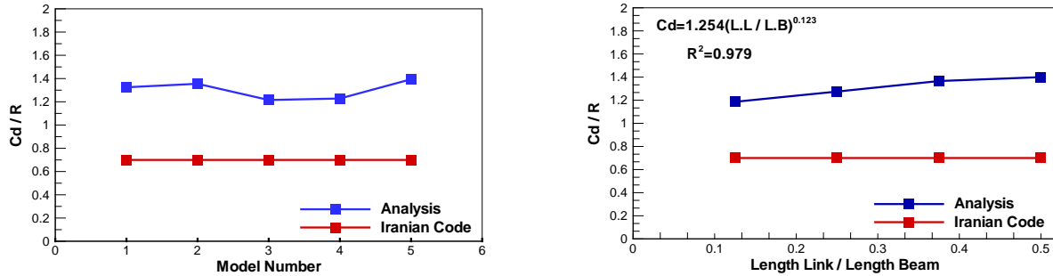
Fig 4: Variation of DRF ratio concerning (a) Bracing kind of spans (b) Length of link beam.
