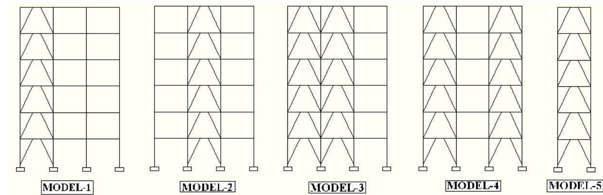
Fig 3: Number of bracing models.
