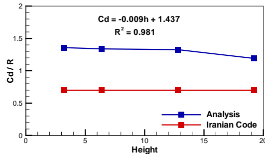
Fig 5: Variation of DRF with height of building.
