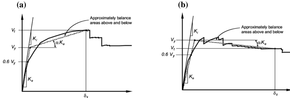
Fig 2: Idealized force displacement curves, (a) Positive post-yield slope, (b) Negative post yield slope (FEMA-356).
